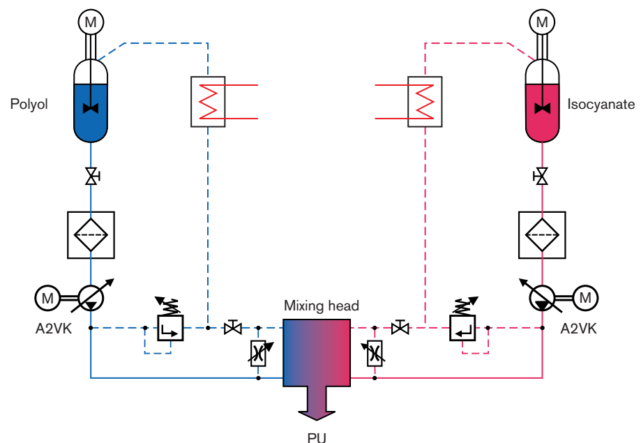
Principle of a PU foaming machine
