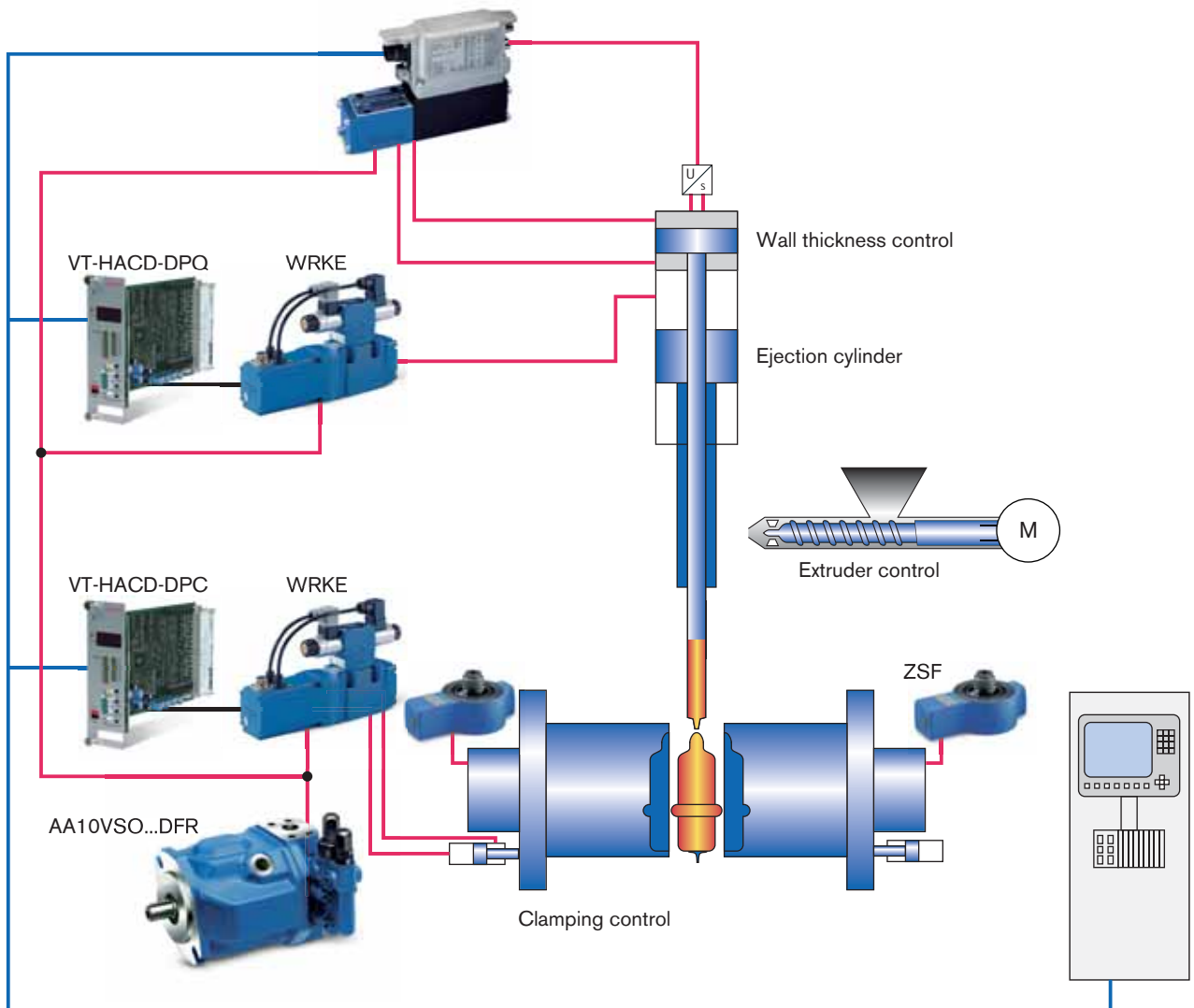
Blow molding machine
