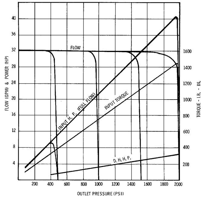
SV-40 @ 1800 rpm
