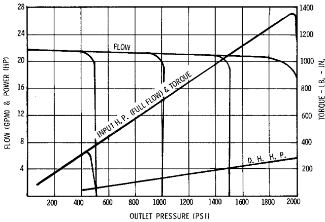
SV-40 @ 1200 rpm
