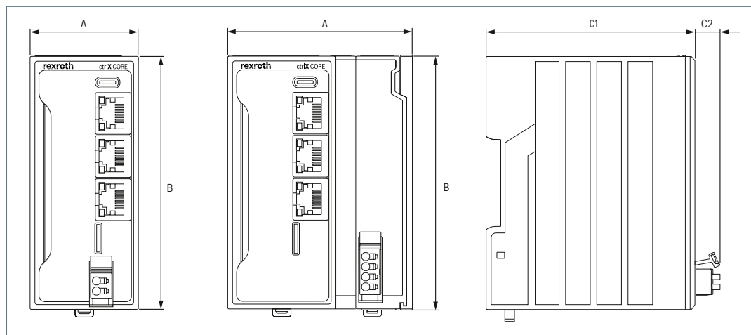
ctrlX CORE X3
