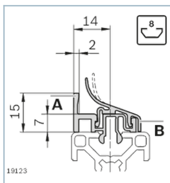
Protective pane profile, clean room, N10 modular dimensions 40
