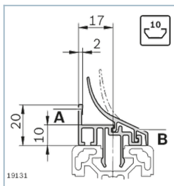
Protective pane profile, clean room, N10 modular dimensions 40
