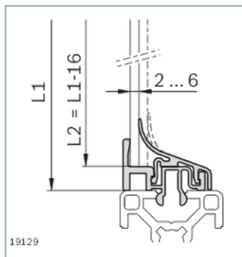
Protective pane profile, clean room, N8
