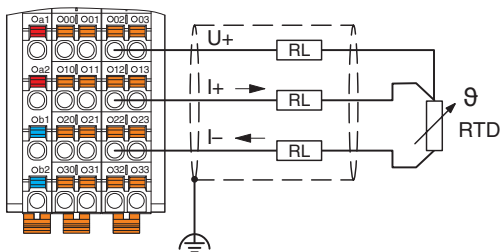
Fig. 4 Connection example: 3-conductor connection
