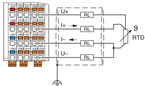
Fig. 6 Connection example: 4-conductor connection for 3-conductor sensor with very long supply lines (> 100 m)
