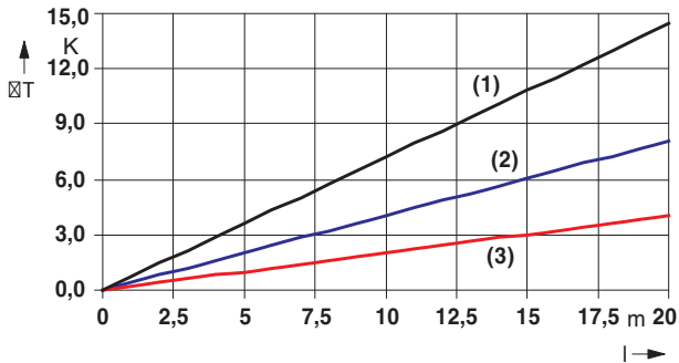
Fig. 8 Systematic temperature measuring error \Delta T depending on the cable length l
