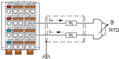
Fig. 5 Connection example: 2-conductor connection
