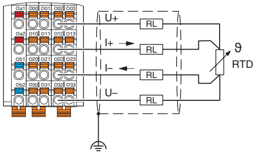
Fig. 3 Connection example: 4-conductor connection
