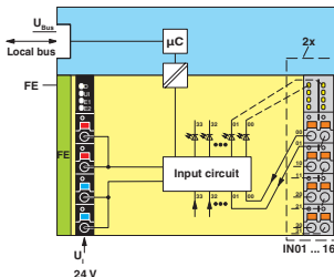
Fig. 1 Internal wiring of the terminal points
